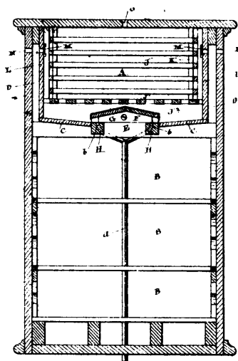
17657 Alexander's Refrigerators.
