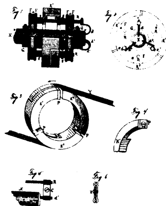
17661 Thomson's Commutators.
