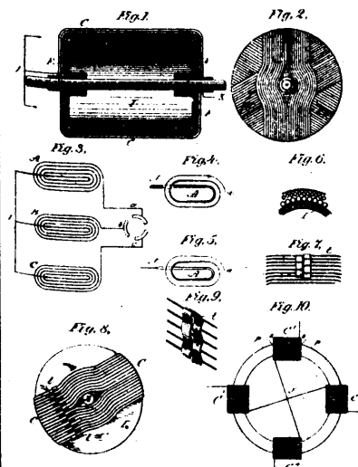
17662 Thomson's Generators.
