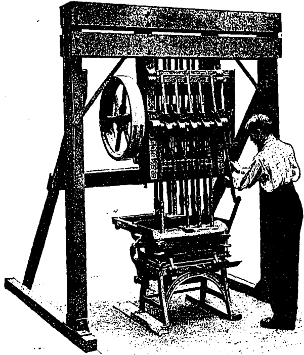
The "IDEAL" Automatic Tamber. Makes blocks quicker (capacity 500 to 600 blocks per day), makes them better—stronger, more dense, and more impervious to moisture. SPEED, COMBINED WITH LABOR-SAVING DEVICES, ARE THE GREATEST TENDENCIES TO SUCCESS.
