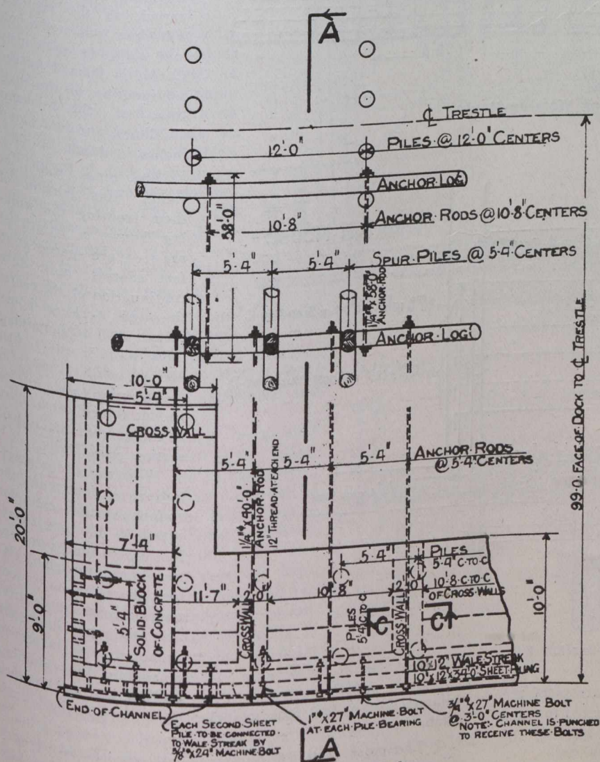
Fig. 3.—Plan at Inshore End.
