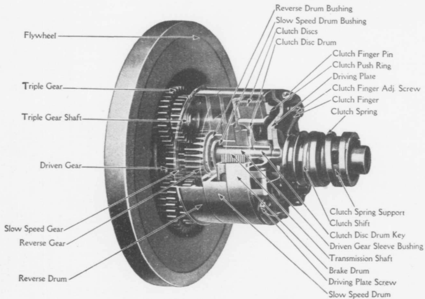
Transmission, showing all gears in mesh. (Cut No. 14)
