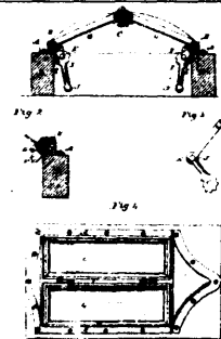
9191 Wood &amp; Washburn's Improvement on Car Windows.
