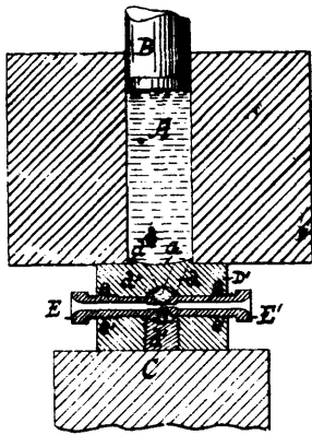
26949 Robertson's Hydraulic Press for Coating Wire, etc., with Lead.
