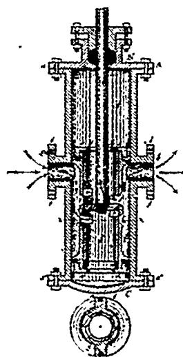
26099 Powers' Force Pump.
