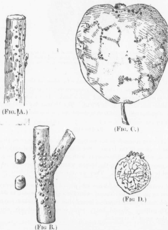
A and B, portions of branches infested; C, a pear infested; D, larva of female enlarged.
