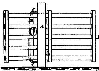
4716 Brown's Improvements on Farm Gates.
