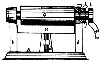
4718 Weston's Improvements on Photograph Burnishers.
