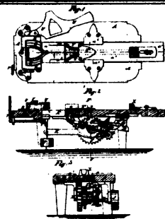
4709 Higgins' Machine for Bending Wood for the Handles of Shovels, &amp;c.
