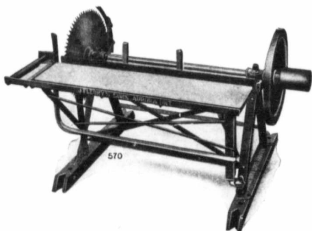
Fleury's Circular Saw Machine No. 3
