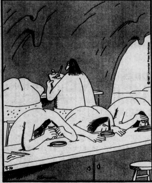
Early microbiologists
