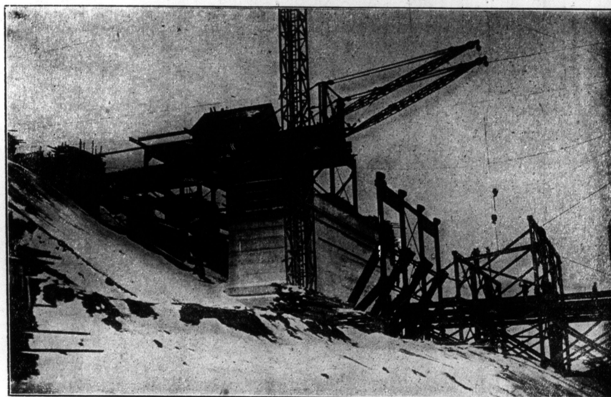
Large construction gang is placing steel work of Bloor street viaduct.
