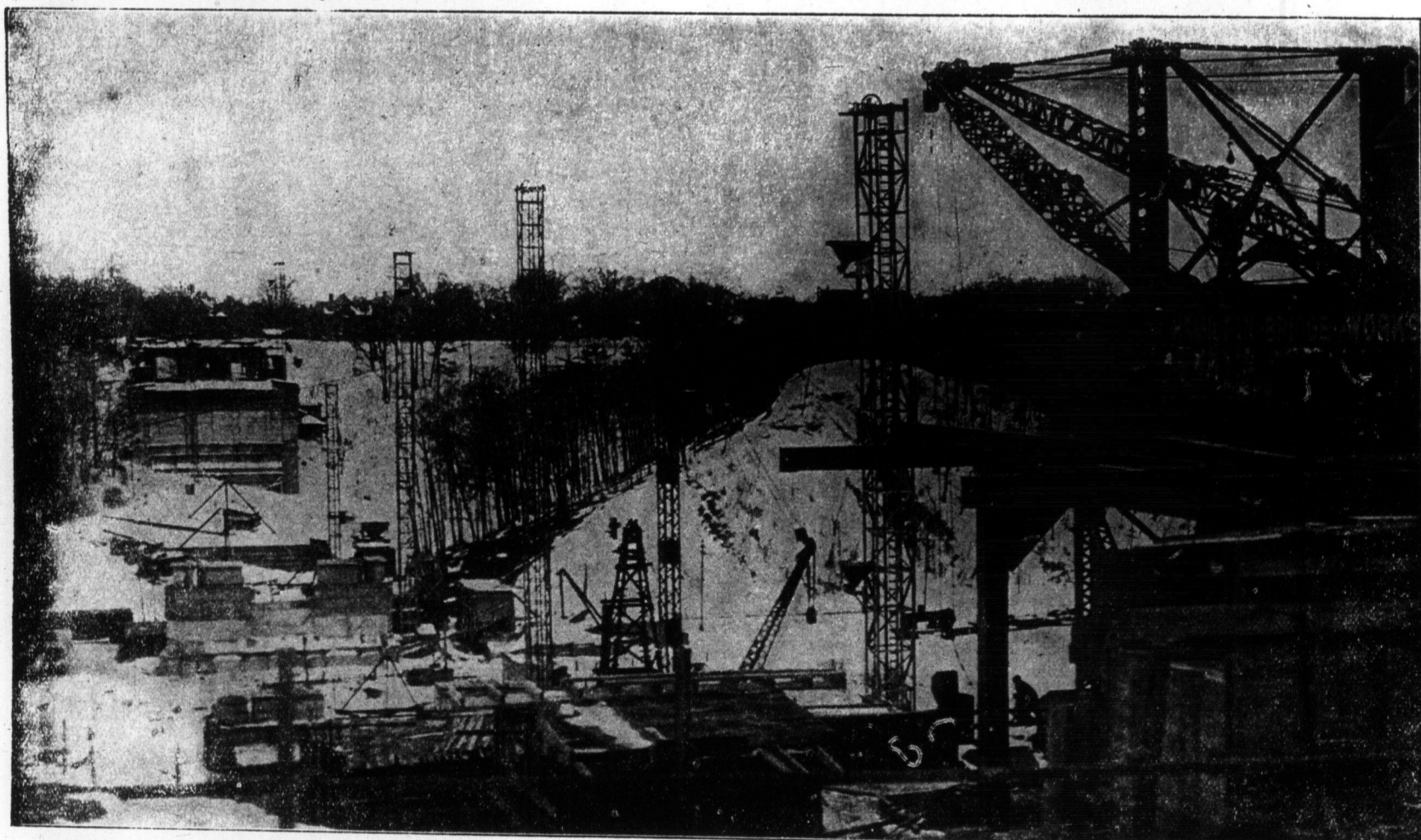
Rushing work on the new Bloor street viaduct. One of many views showing the progress of this important civic improvement.
