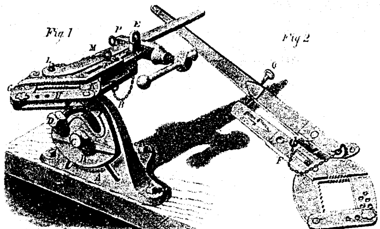
NEAMES' COMBINED PIPE WRENCH AND VICE.
