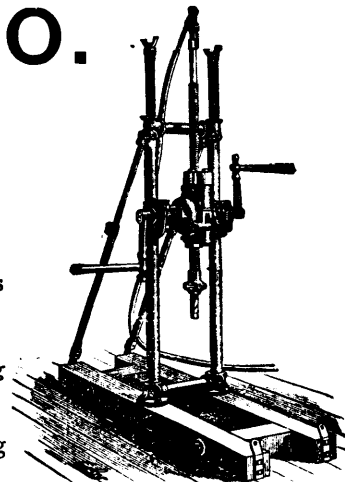
"Bravo" Hand Power Drill. Capacity. 400 feet. 1 3/4" hole 12-16"
