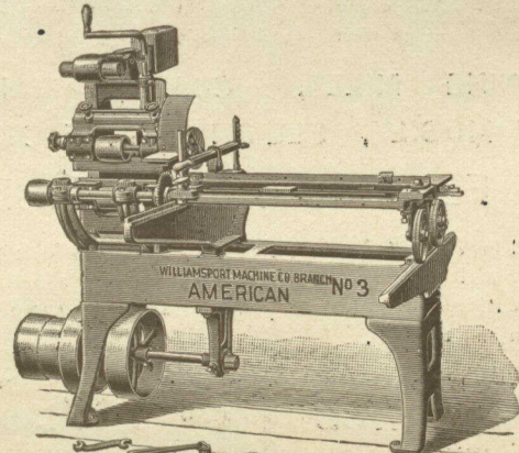
TENONER
