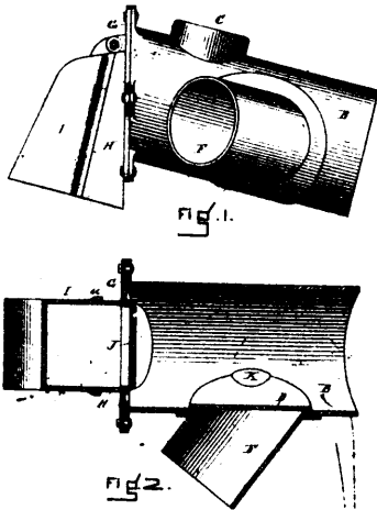
34592 Higgins' Sewer Trap.
