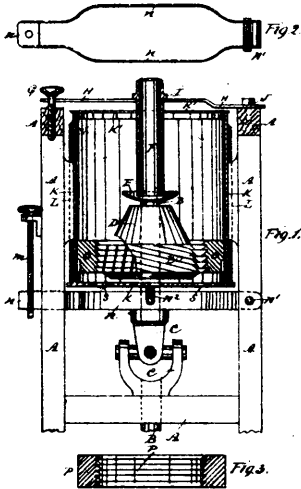
34588 St. Denis' Wheat Breaking Machine.
