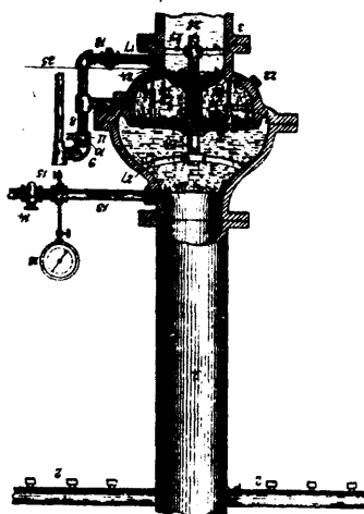
27862 Grinnell's Fire Extinguishing apparatus
