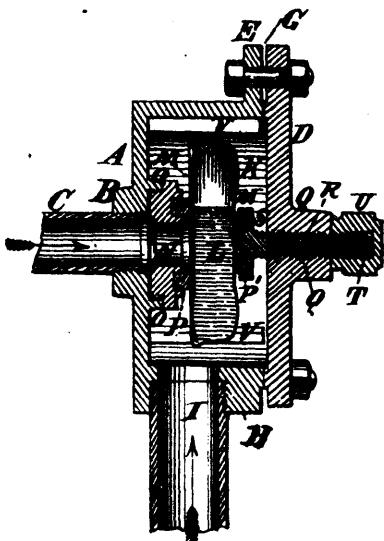
27855 Gold's Steam Trap.
