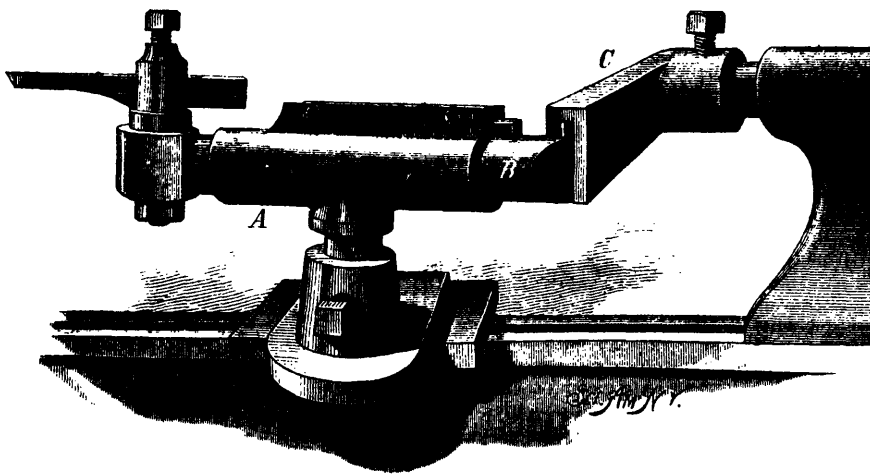
Fig. 4.—BORING ATTACHMENT.
