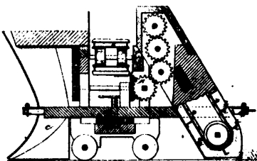
7737 Jensen's Snow Plough and Track Clearer.
