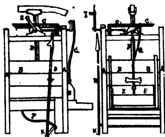
7747 Davis' Improvement on Brick Machines.
