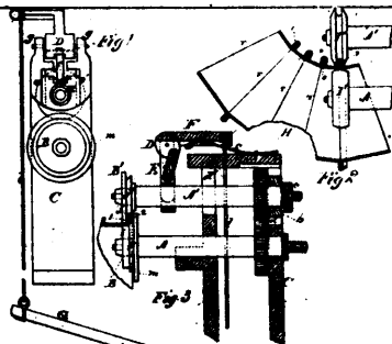
7741 Amana's Stove-pipe Elbow Machine.
