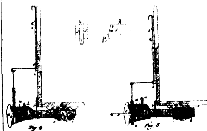
2084 Forrest's Car-Coupler.
