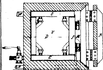
2072 Warner's Fire-proof Vault.
