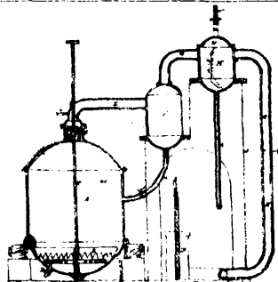
2078 Steers' Apparatus for Manufacturing Dye and Saccharine Salts.
