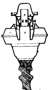
2081 White &amp; Knight's Lamp.
