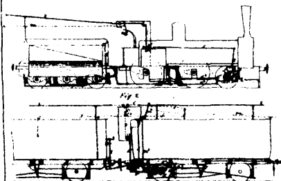
2079 Heberlein's Railway Car-Brake.
