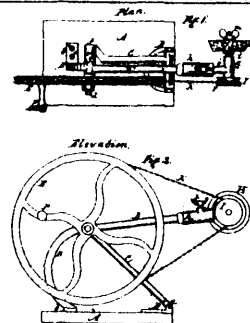
2076 Curran's Harvesting Machine Sickle Grinder.
