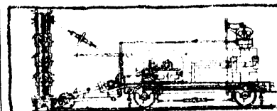
2087 Beaumont &amp; Appleby's Rock or Stone Drilling and Tunnelling Apparatus.
