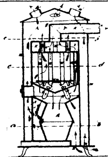
2075 Gray's Heating Stove.
