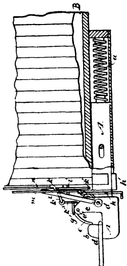
42085 Smith's Car Coupler.
