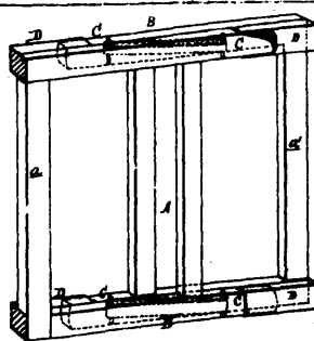
3709 Kellam, Hayes &amp; Hayes's Improvements on Window Screen Frames.
