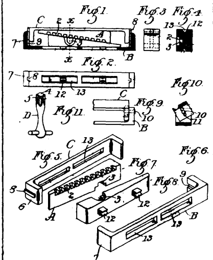
37426 Mowers' Printers' Quoins.
