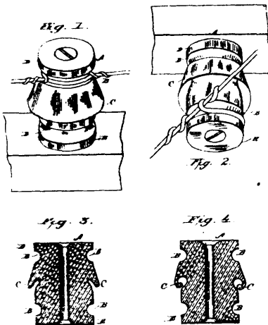
37418 Bertollet's Electric Wire Insulator.
