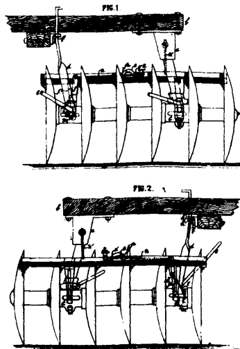
37419 Patton's Waggon Brake.
