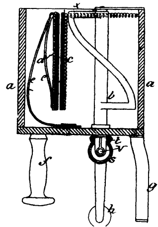
37420 Nilsson's Milking Apparatus.
