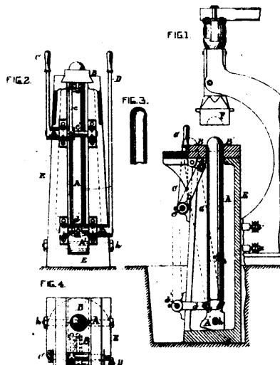
31832 Kennedy's Machine for Closing Metal Tubes.
