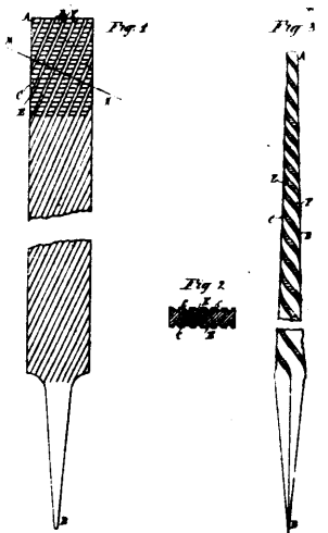
31831 Leclercq's Manufacture of Files, etc.
