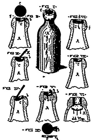
24258 Painter's Bottle Stopper.
