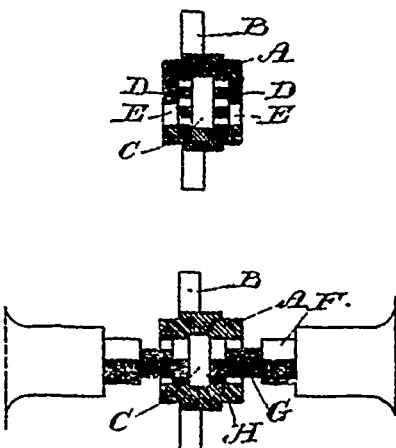
24257 Alvoni's Knob Attachment.
