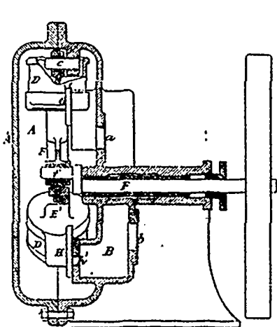
24254 Schouheyden's Fluid Pressure Engine.
