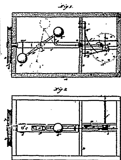
24259 Herdon's Centrifugal Speed Indicator.
