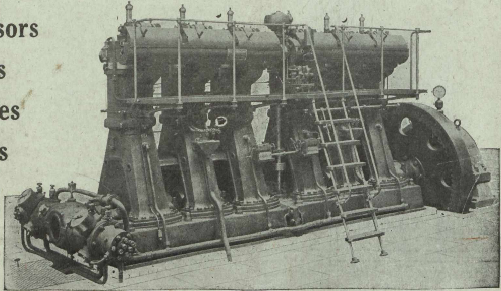
BELLISS & MORCOM DIESEL CRUDE OIL ENGINE.
