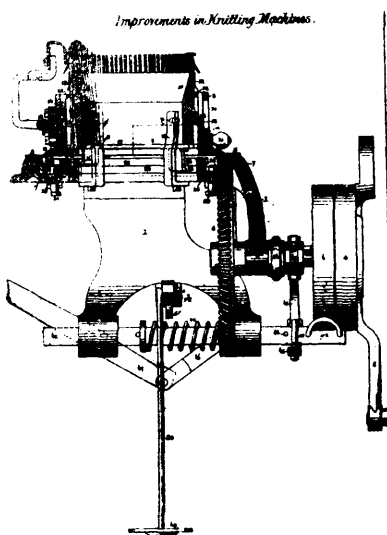
34119 Franck's Knitting Machine.
