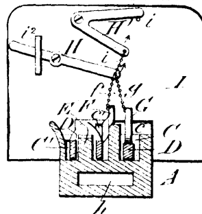
13615 Blanchard's Improvements on Car-couplings.
