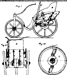
13598 Liedman & Beger's Apparatus for Imparting Motion to Carriages, Vessels, and other Bodies.
