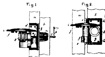
13600 Moore's Improvements on Shutters.
