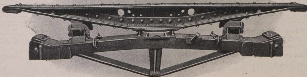
Simplex Body and Truck Bolster and Susemihl Side Bearings.
