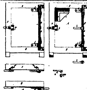
4358 Taylor's Improvements on Burglar Proof Safes.
