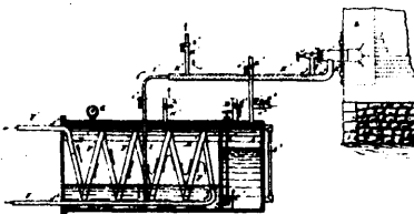
4356 Robinson's Apparatus for Oil Burning Furnaces.
