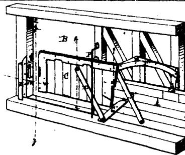
4354 Van Liew's Grain Door for Freight Cars.
