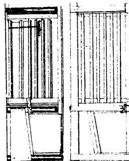
2057 Spencer's Counterpoise Farm Gate.
