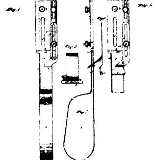
2051 Nunn's Sewing Machine Tuckor.
