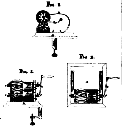
31007 Robertson's Knife, Fork and Spoon Scourer.
