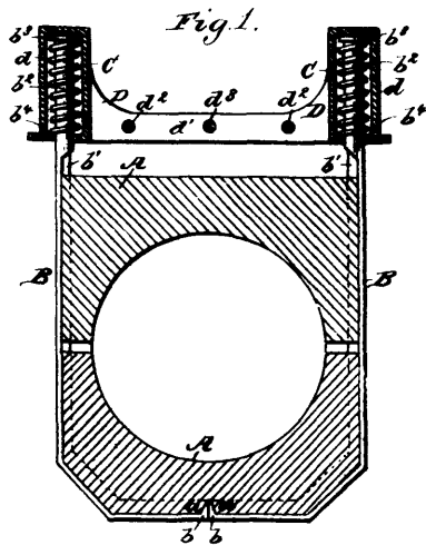
31005 Sweeney's Dust Guard.
