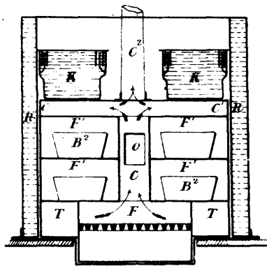
31006 Tomkins' Portable Cooking Apparatus.
