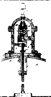
14075 Wilson's Combined Low Water Alarm and Safety Valve for Steam Boilers.
