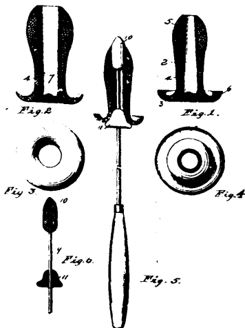
36900 Lyford's Impregnator for Veterinary Use.
