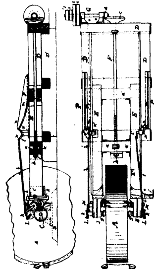
18366 Trier's Machine for Manufacturing Grindstones.
