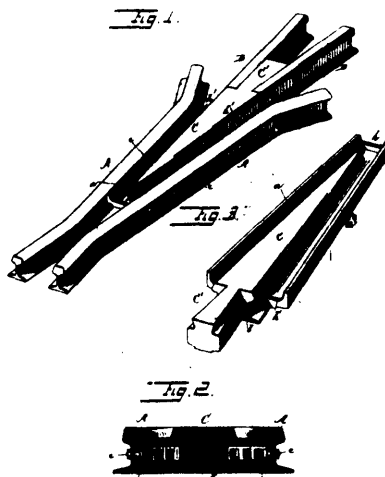
18359 Morden's Railway Frog.
