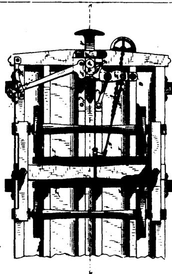
18363 Rote's Car Brake.
