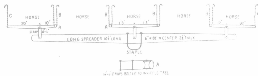
Evener for driving five horses abreast on rank row or harness.
