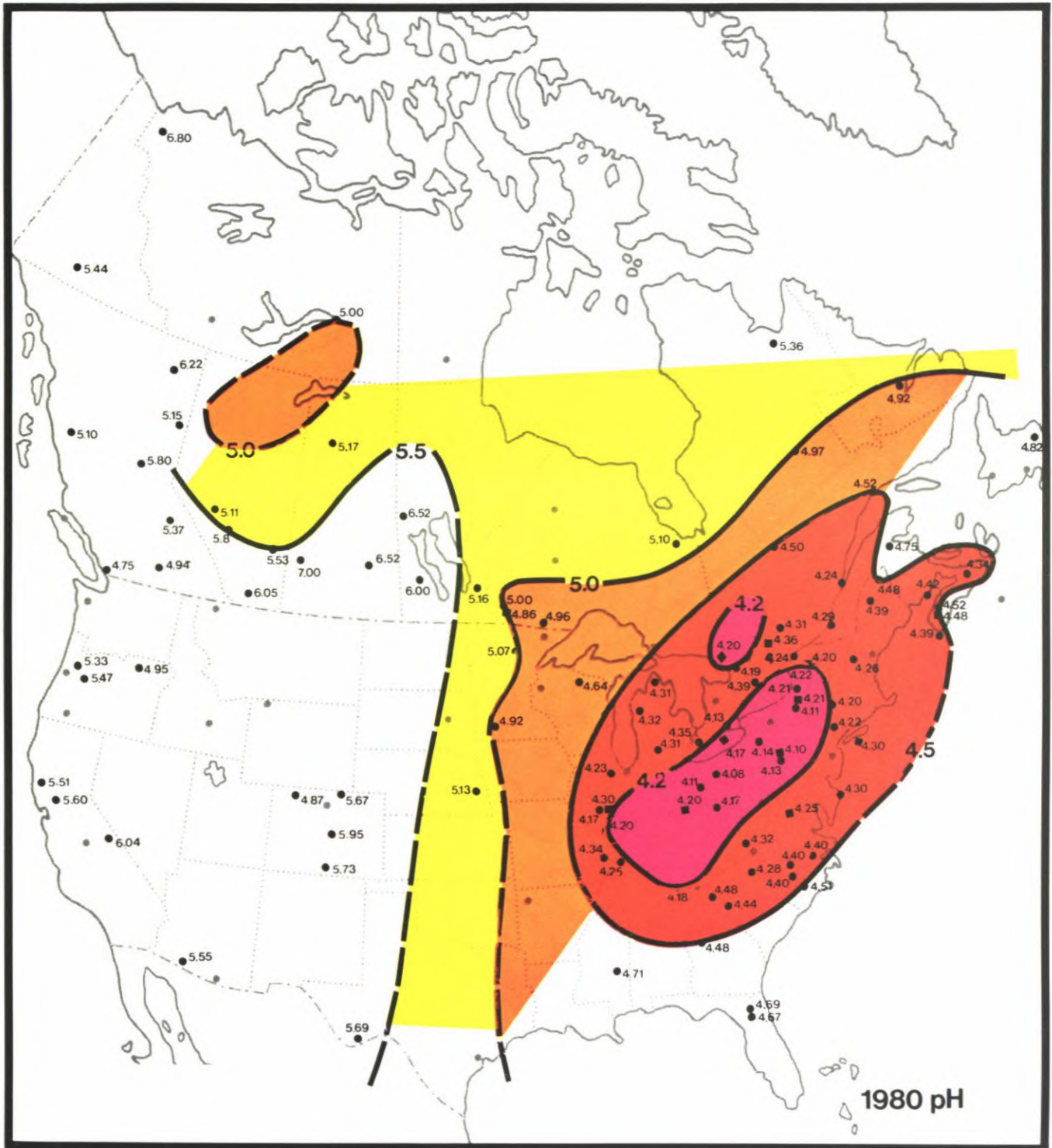
Precipitation amount- weighted mean annual pH in North America for the calendar year 1980
