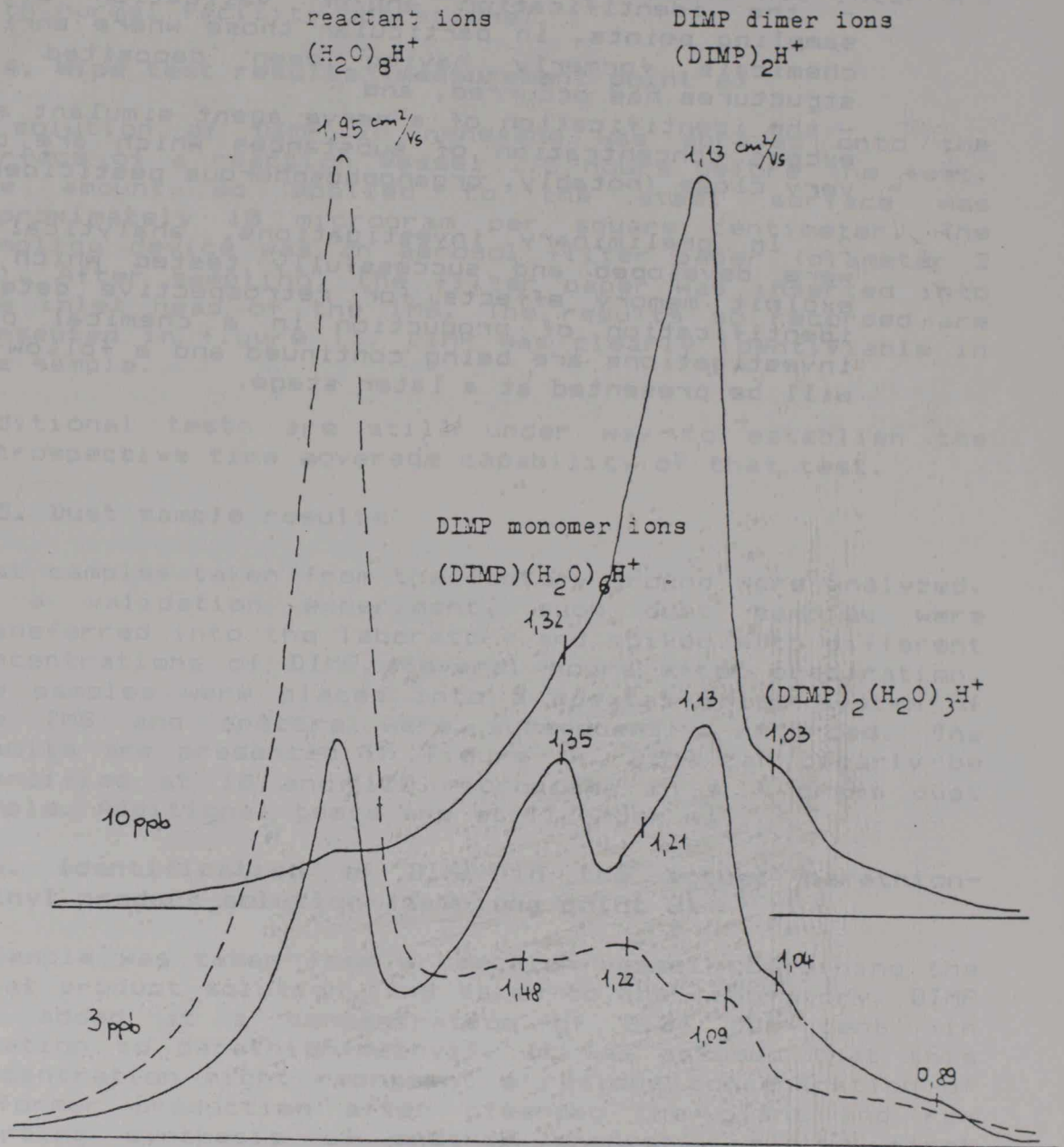
Fig. 1: IMS spectra recorded for 3 and 10 ppb DIMP in air
