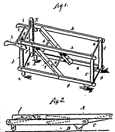
24622 Taft's Machine for Lifting Waggon, etc.
