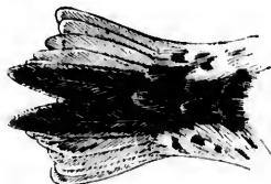
Tringa maculata. Tail and upper tail coverts.
