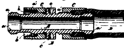
18131 Chadwick's Improvements in Hose Couplings.
