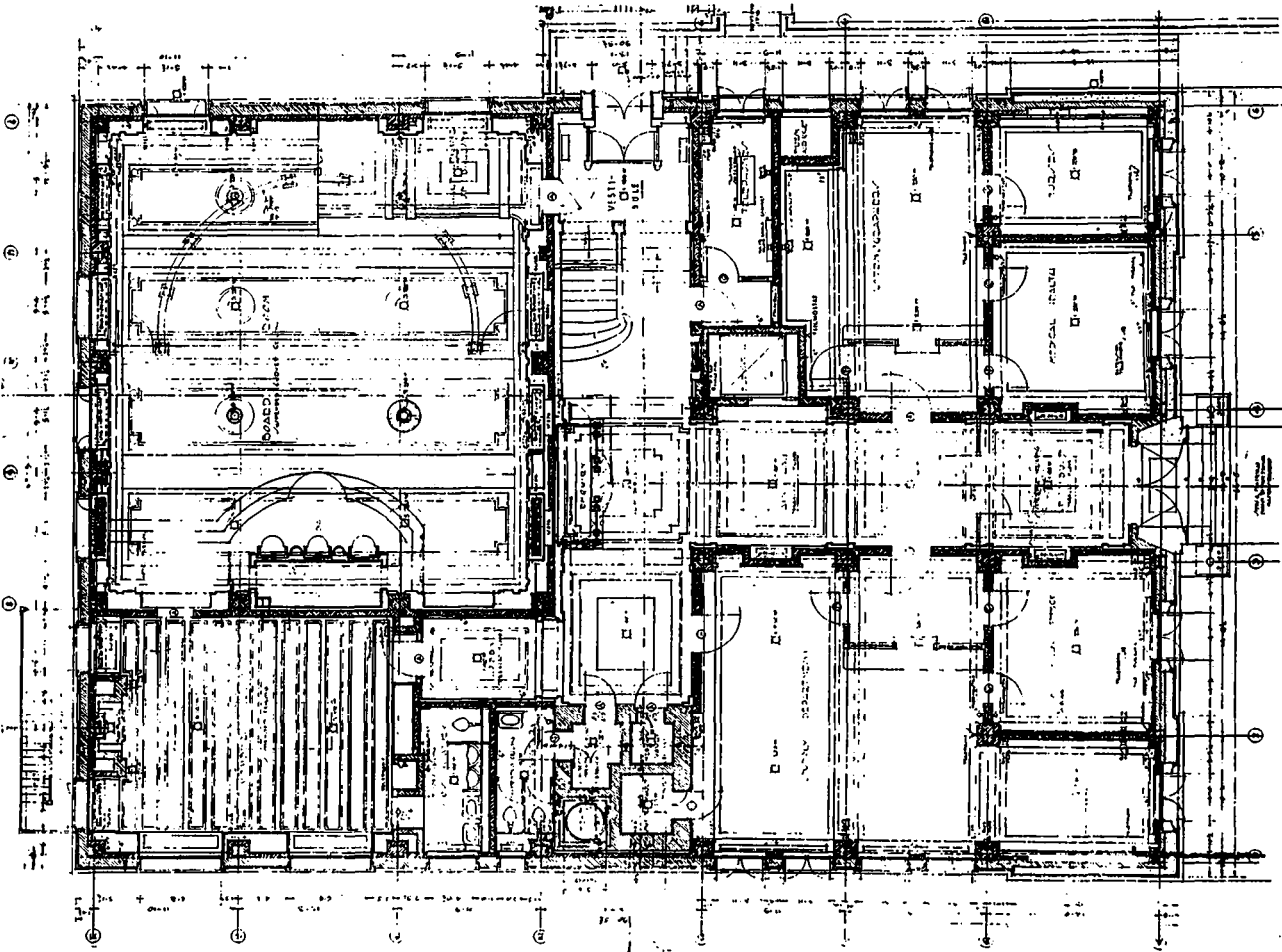
GROUND FLOOR PLAN OF ADMINISTRATION BUILDING.
