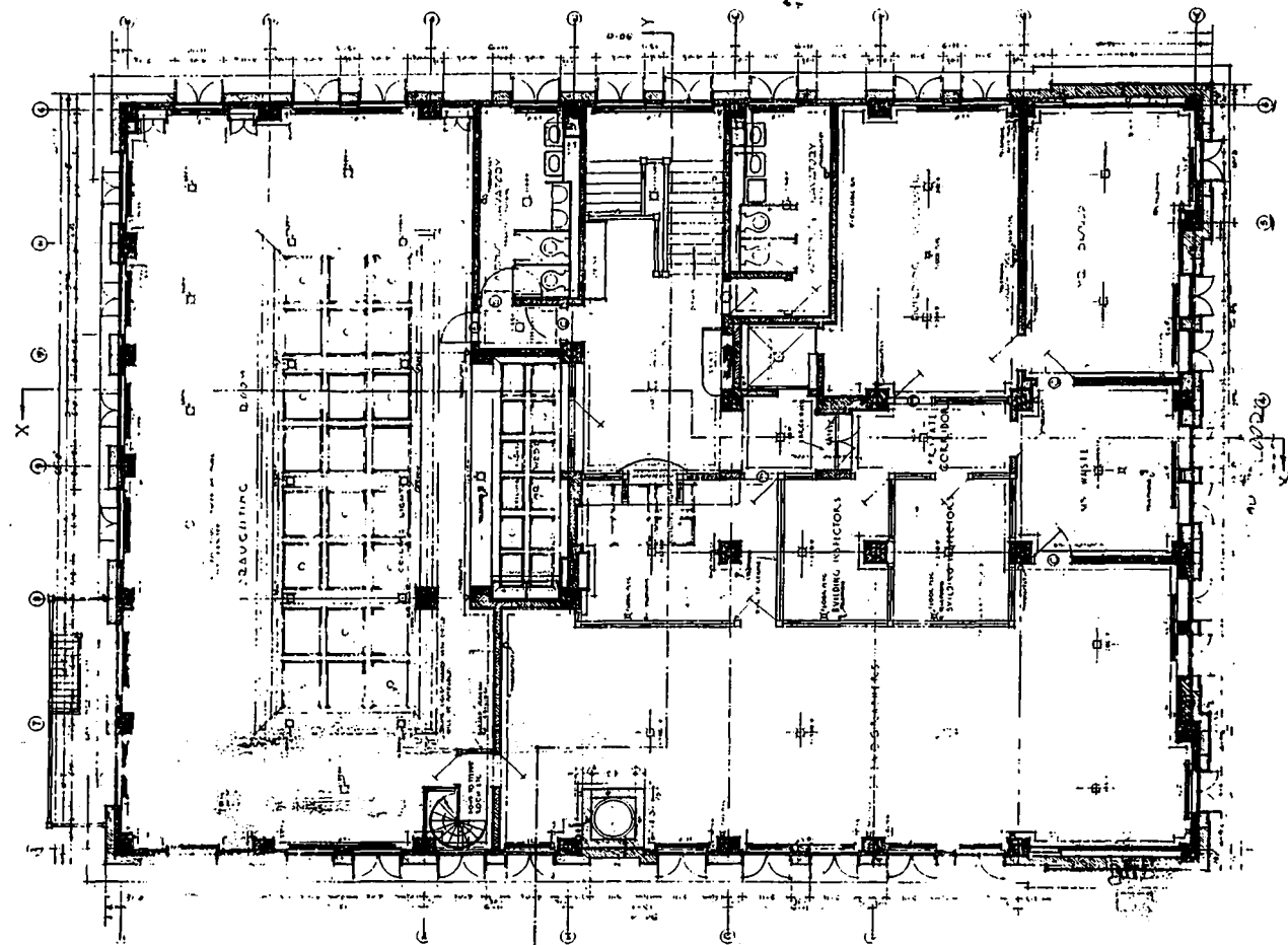
FOURTH FLOOR PLAN OF ADMINISTRATION BUILDING.
