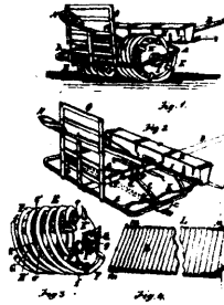
8531 Nichols' Improvements in Rotary Harrows.
