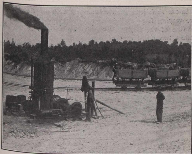
Fig. 4. Stationary Engine Hauling Cars.
