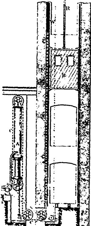
Fig. 6. Hydraulic Jigger Lift, vertical cylinder, high pressure.
