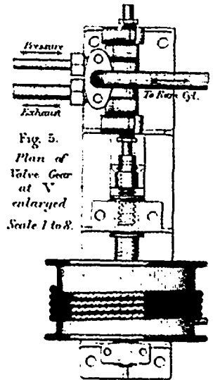
Hydraulic Jigger Lift, horizontal cylinder.
