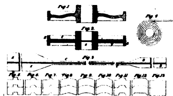
5995 Krupp's Construction of Railway and other Wheels.
