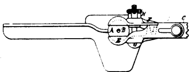
5990 Bradley's Improvements in Harvesters.
