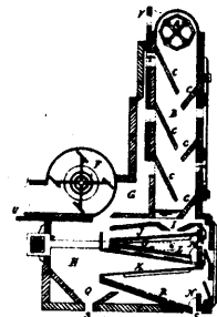
5986 Bodwell &amp; Scott's Machine for Fastening Lock Gates.
