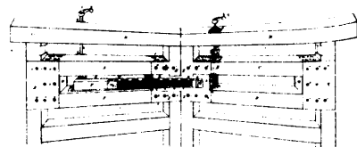
5986 Bodwell &amp; Scott's Machine for Fastening Lock Gates.
