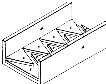
2386 Brewer's Chute and Fish Way.
