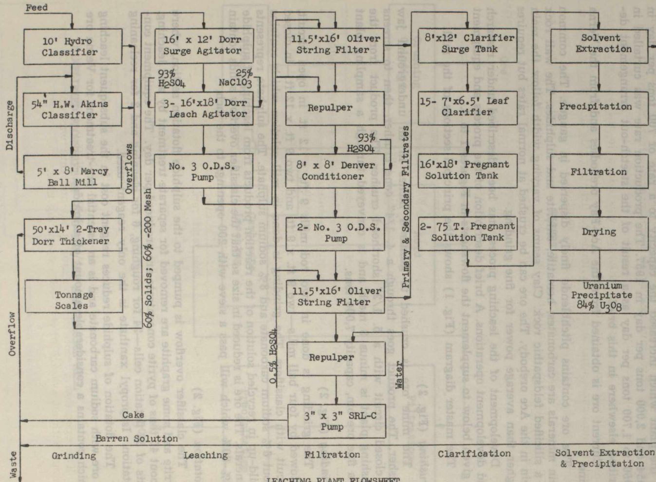
LEACHING PLANT FLOWSHEET (300 TPD - 1/2 Current Gravity Plant Tailings + 1/2 Reclaimed Tailings)
