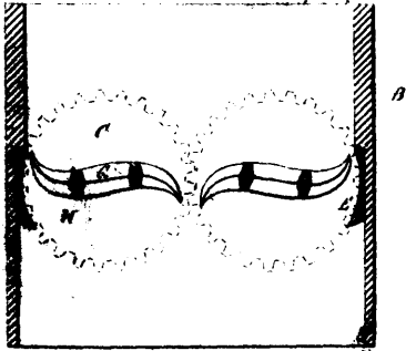
9499 McClave's Improvements on Stove Grates.
