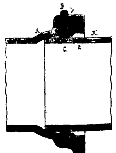
9508 Painter's Method of Forming Joints in Gas and Water Mains.
