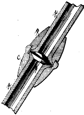
37832 Smith and McPherson's Pipe Coupling.
